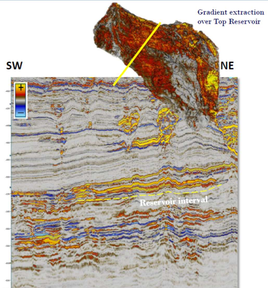
AVO Gradient overlaid on Ufar stack
